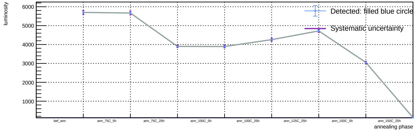
Sensor A1, v = 5 V, T = 23 °C - Spot 3: luminosity vs phase
