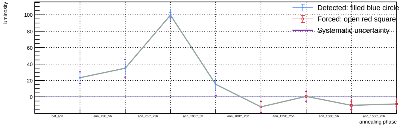
Sensor A1, v = 5 V, T = 23 °C - Spot 30: luminosity vs phase
