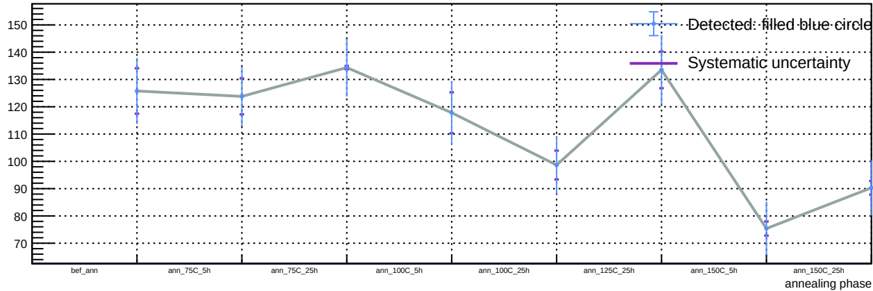
Sensor A1, v = 5 V, T = 23 °C - Spot 31: luminosity vs phase
