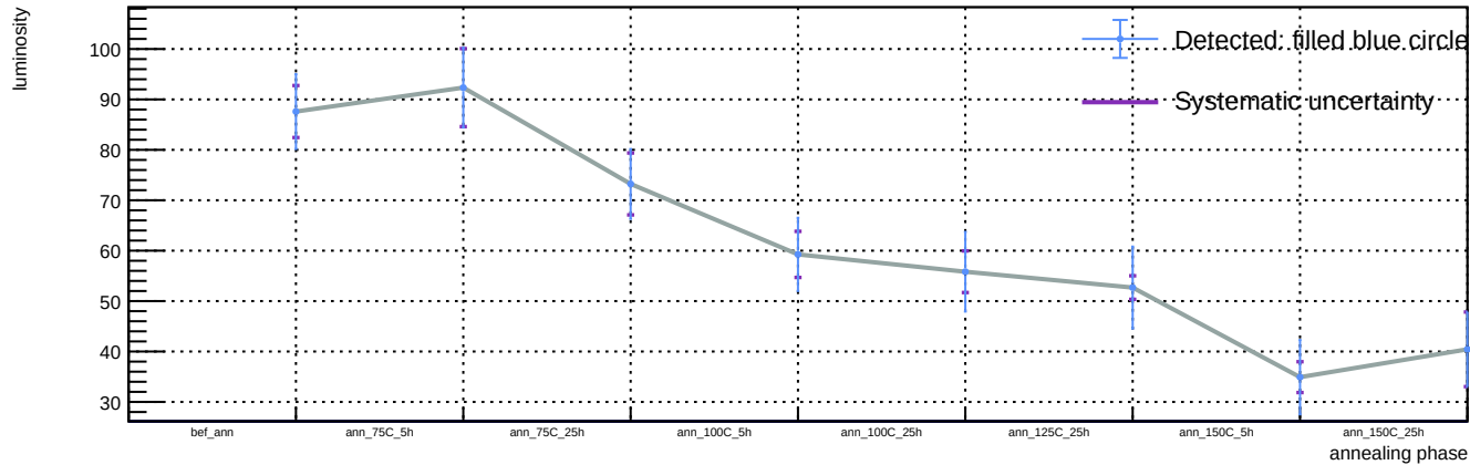
Sensor A1, v = 5 V, T = 23 °C - Spot 32: luminosity vs phase
