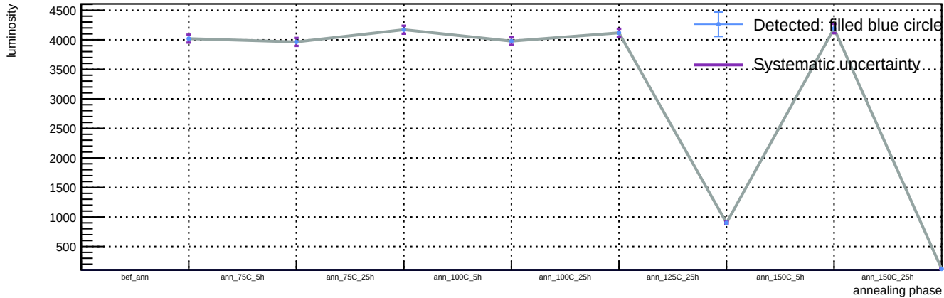
Sensor A1, v = 5 V, T = 23 °C - Spot 33: luminosity vs phase
