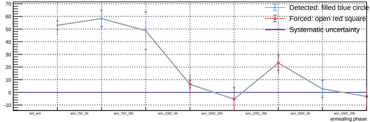
Sensor A1, v = 5 V, T = 23 °C - Spot 34: luminosity vs phase
