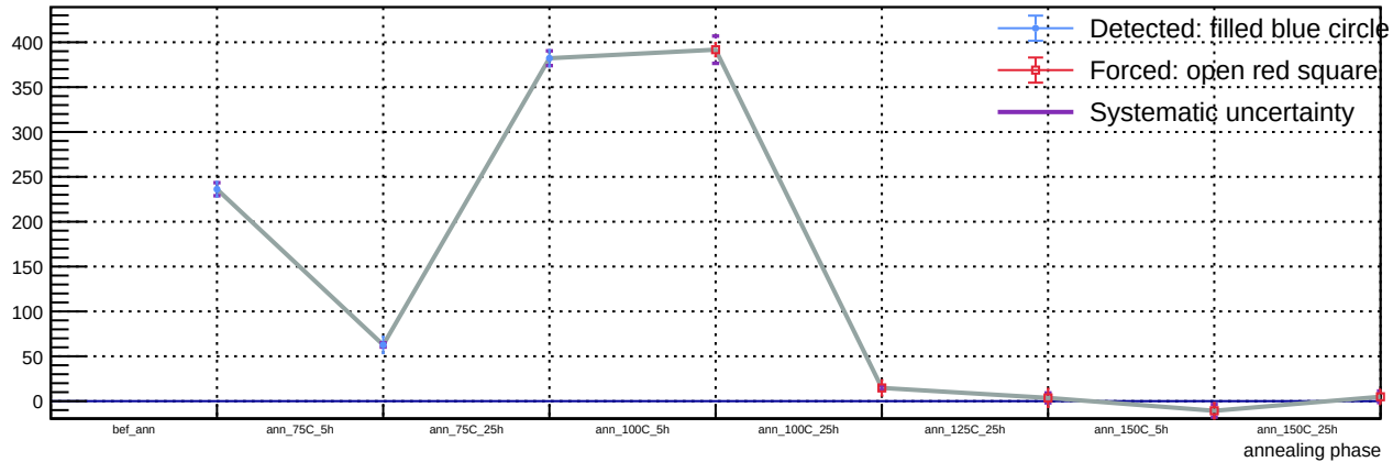
Sensor A1, v = 5 V, T = 23 °C - Spot 35: luminosity vs phase
