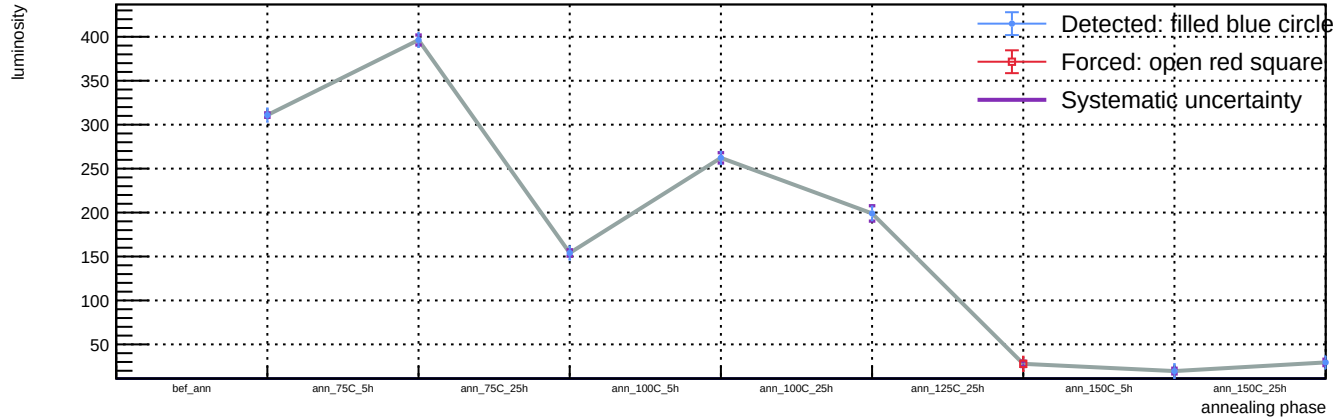
Sensor A1, v = 5 V, T = 23 °C - Spot 37: luminosity vs phase
