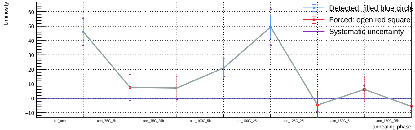
Sensor A1, v = 5 V, T = 23 °C - Spot 38: luminosity vs phase
