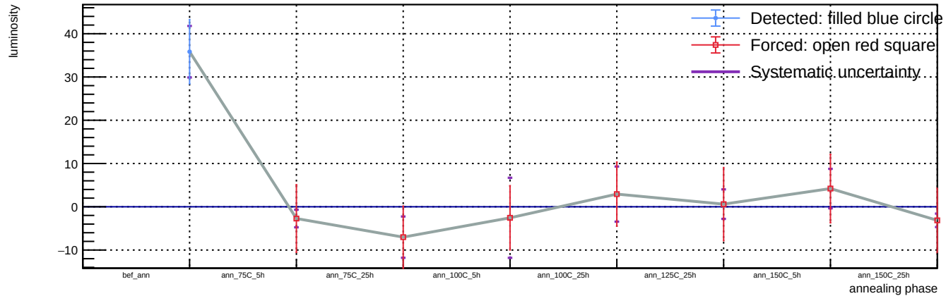
Sensor A1, v = 5 V, T = 23 °C - Spot 39: luminosity vs phase
