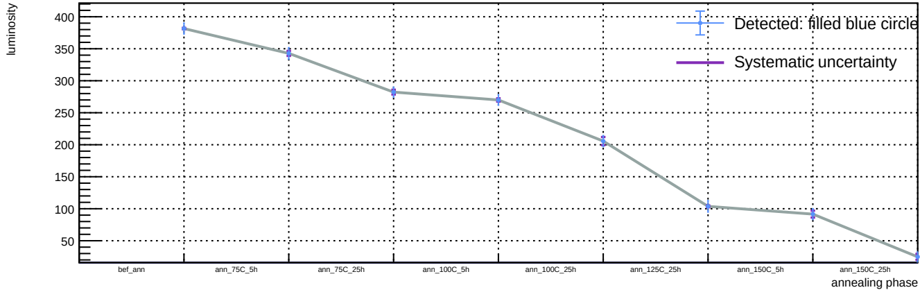
Sensor A1, v = 5 V, T = 23 °C - Spot 4: luminosity vs phase
