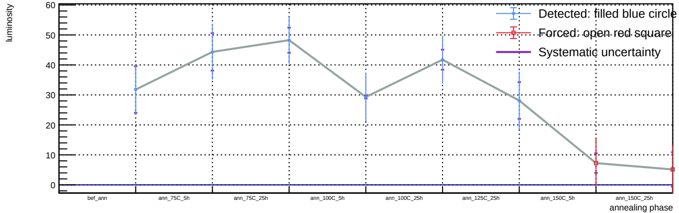
Sensor A1, v = 5 V, T = 23 °C - Spot 40: luminosity vs phase
