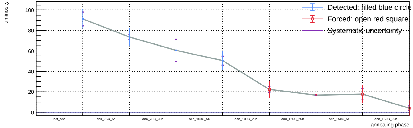
Sensor A1, v = 5 V, T = 23 °C - Spot 41: luminosity vs phase
