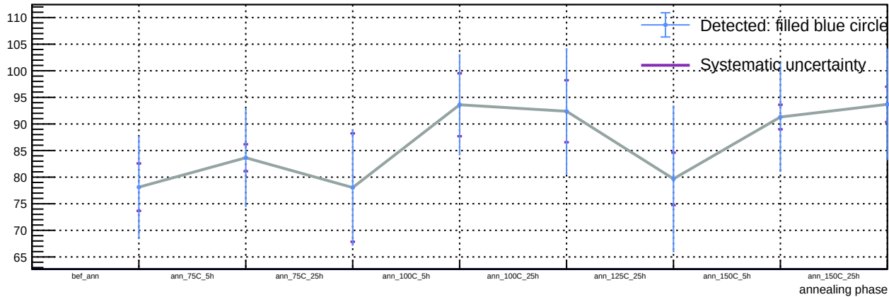
Sensor A1, v = 5 V, T = 23 °C - Spot 42: luminosity vs phase
