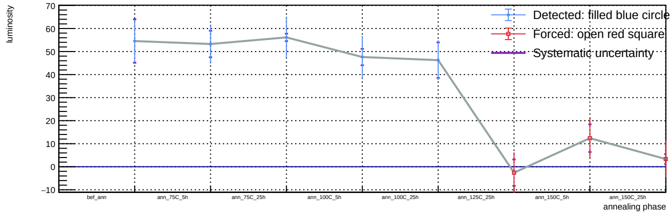
Sensor A1, v = 5 V, T = 23 °C - Spot 43: luminosity vs phase
