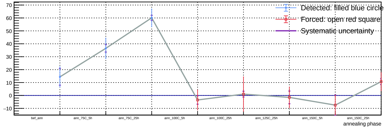
Sensor A1, v = 5 V, T = 23 °C - Spot 44: luminosity vs phase
