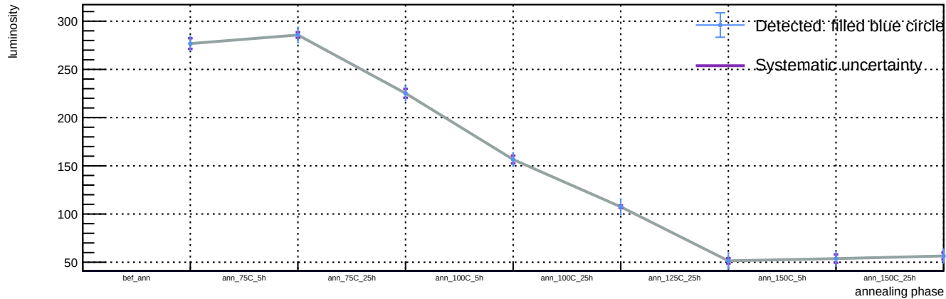
Sensor A1, v = 5 V, T = 23 °C - Spot 45: luminosity vs phase
