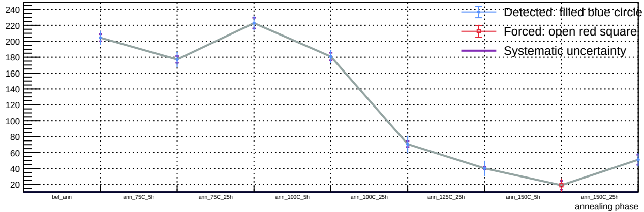
Sensor A1, v = 5 V, T = 23 °C - Spot 46: luminosity vs phase
