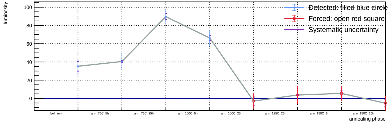
Sensor A1, v = 5 V, T = 23 °C - Spot 47: luminosity vs phase
