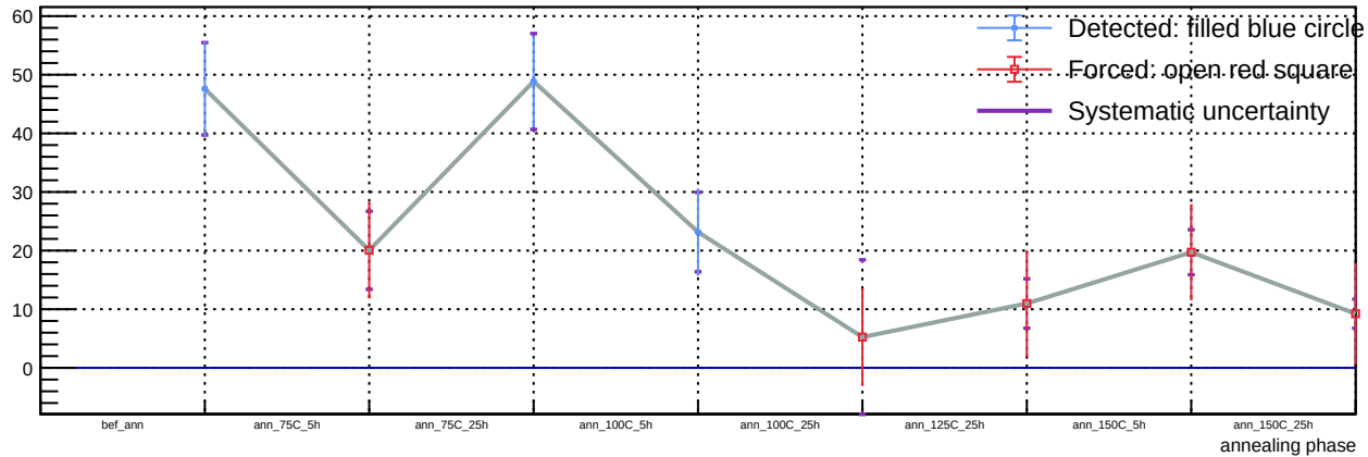
Sensor A1, v = 5 V, T = 23 °C - Spot 5: luminosity vs phase
