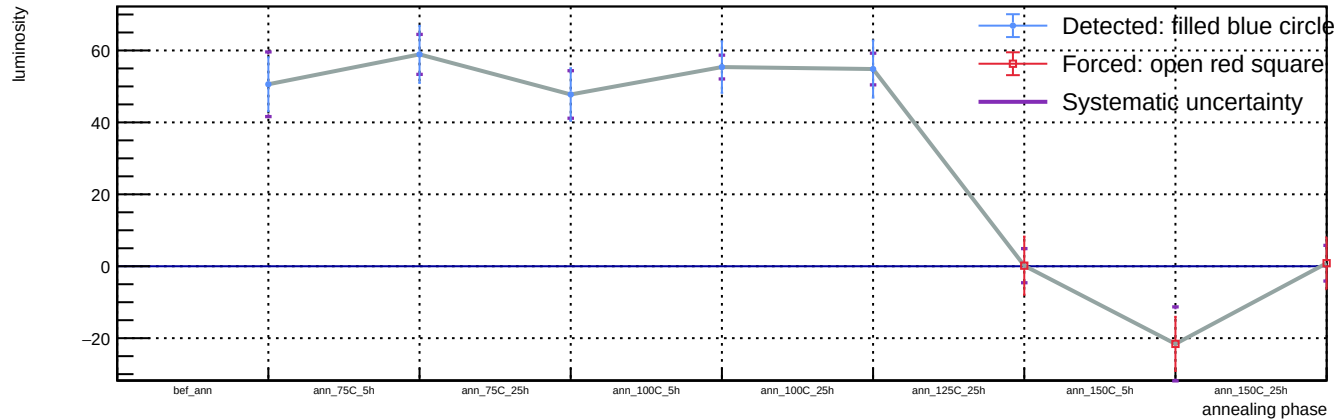
Sensor A1, v = 5 V, T = 23 °C - Spot 50: luminosity vs phase
