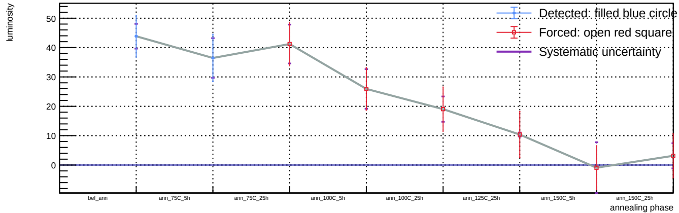
Sensor A1, v = 5 V, T = 23 °C - Spot 51: luminosity vs phase
