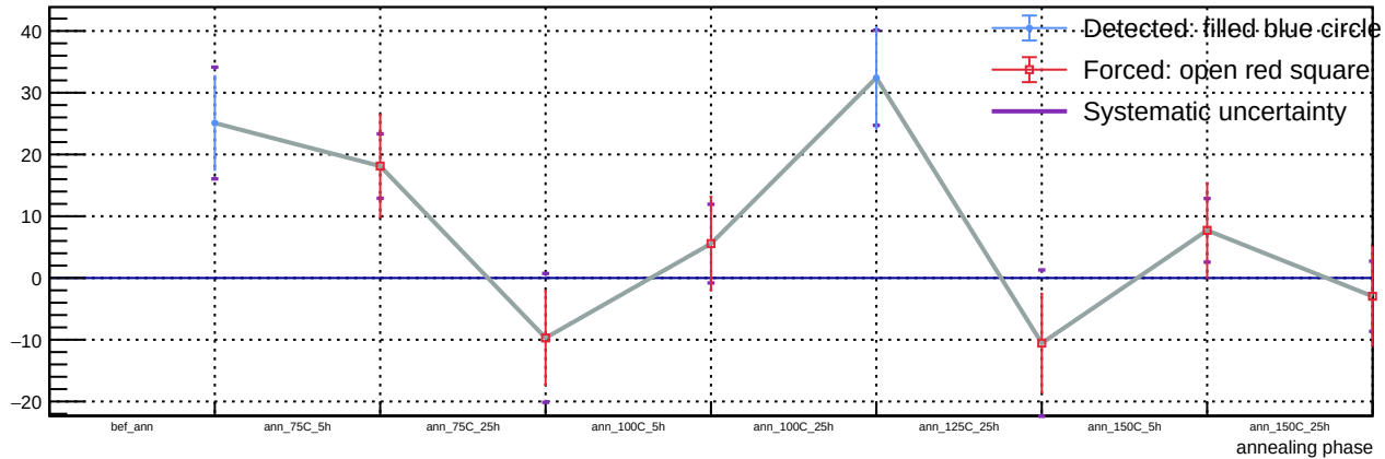
Sensor A1, v = 5 V, T = 23 °C - Spot 52: luminosity vs phase
