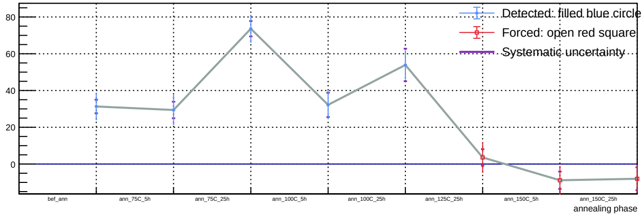
Sensor A1, v = 5 V, T = 23 °C - Spot 53: luminosity vs phase
