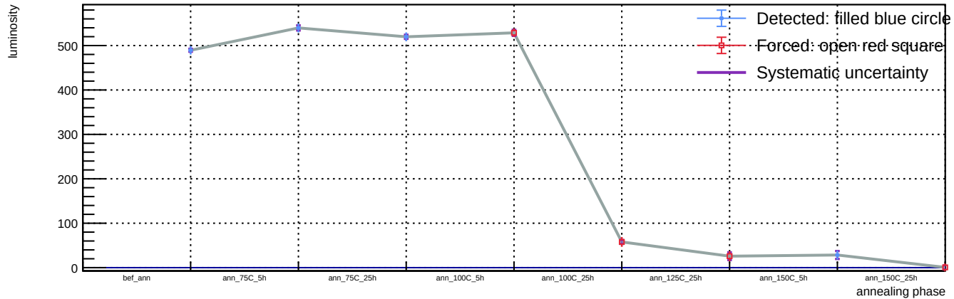
Sensor A1, v = 5 V, T = 23 °C - Spot 55: luminosity vs phase
