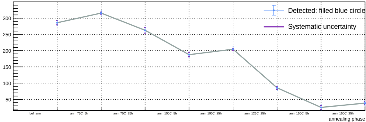
Sensor A1, v = 5 V, T = 23 °C - Spot 56: luminosity vs phase
