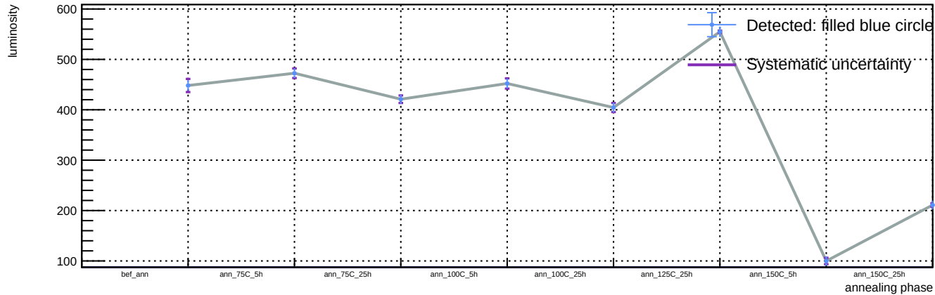
Sensor A1, v = 5 V, T = 23 °C - Spot 57: luminosity vs phase
