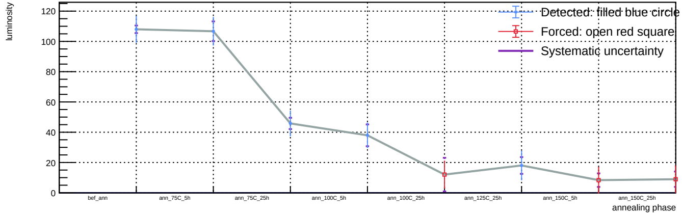
Sensor A1, v = 5 V, T = 23 °C - Spot 58: luminosity vs phase
