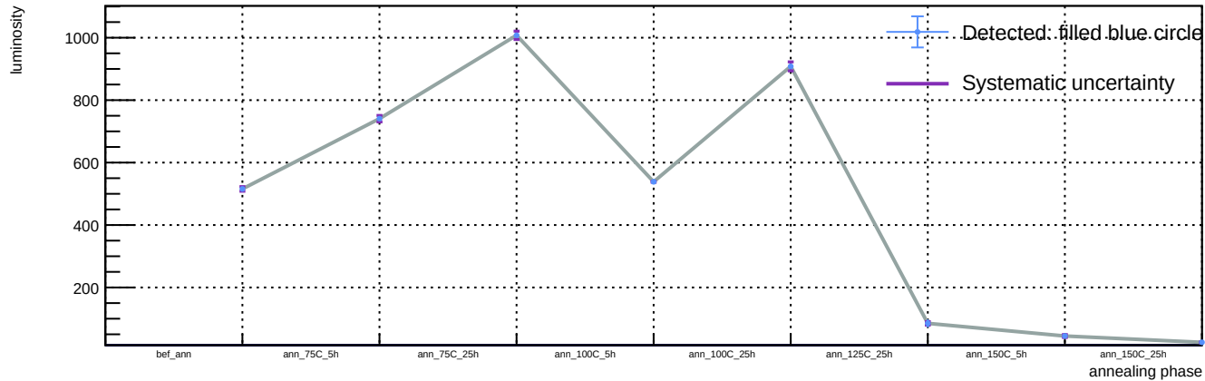
Sensor A1, v = 5 V, T = 23 °C - Spot 59: luminosity vs phase
