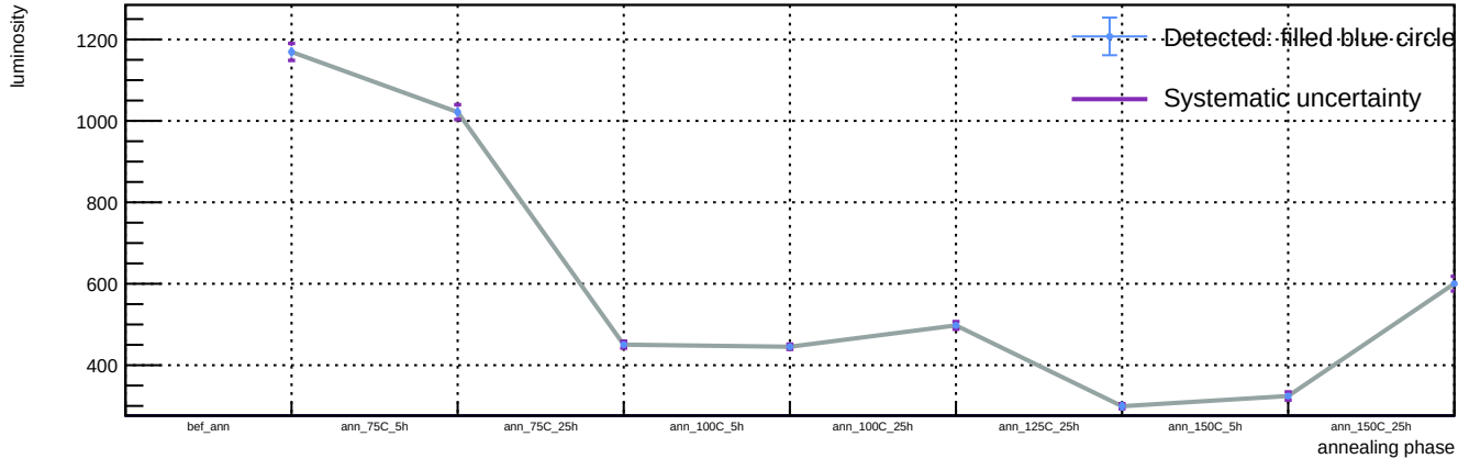
Sensor A1, v = 5 V, T = 23 °C - Spot 6: luminosity vs phase
