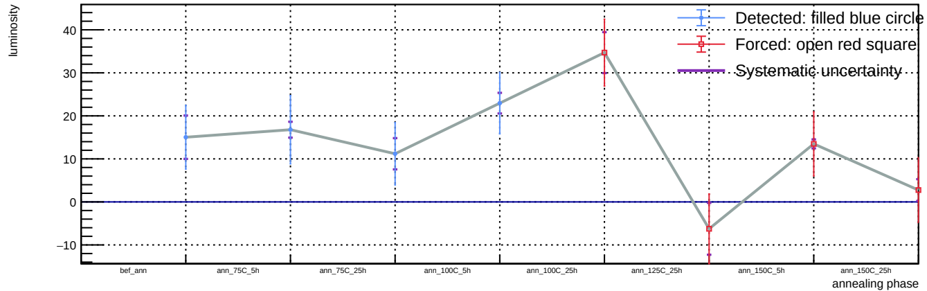
Sensor A1, v = 5 V, T = 23 °C - Spot 60: luminosity vs phase
