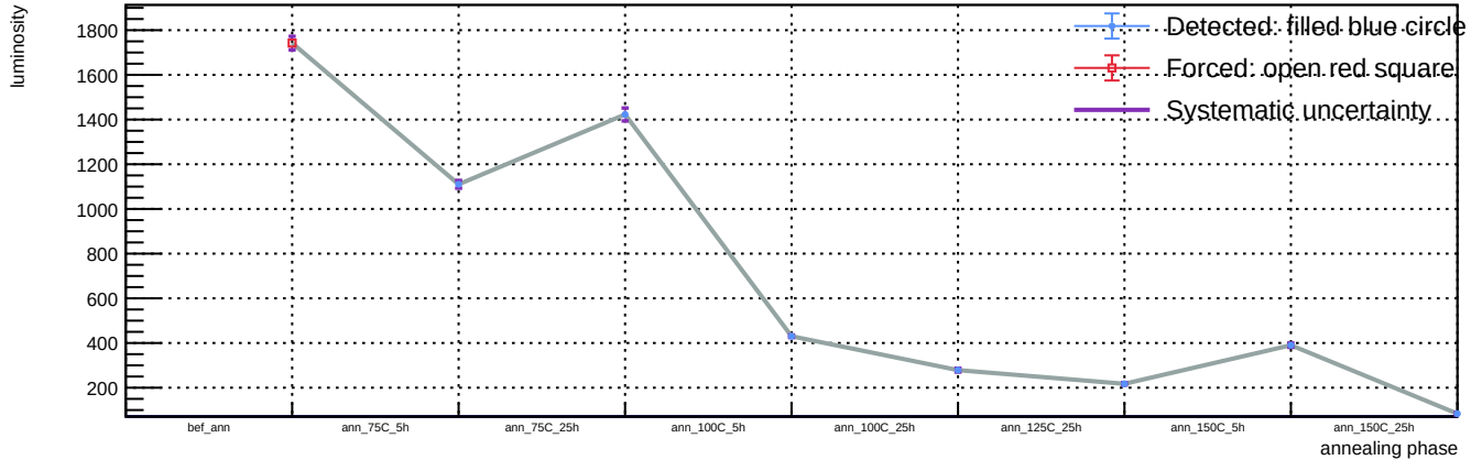
Sensor A1, v = 5 V, T = 23 °C - Spot 62: luminosity vs phase
