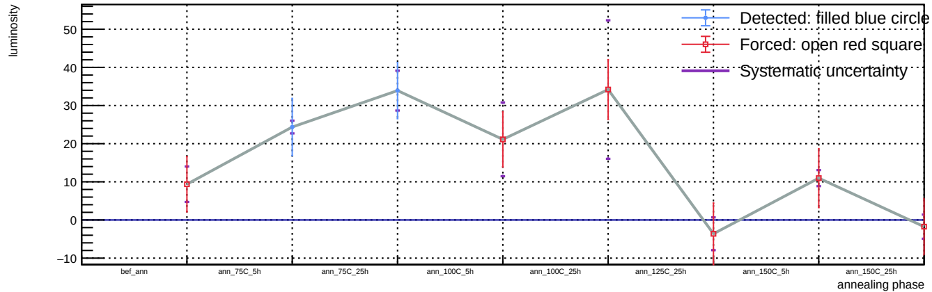
Sensor A1, v = 5 V, T = 23 °C - Spot 63: luminosity vs phase
