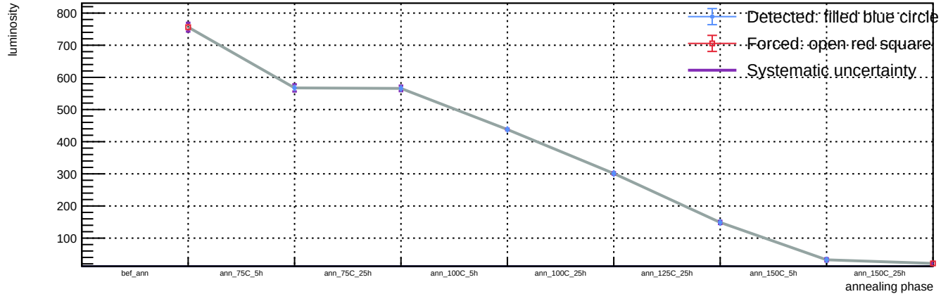
Sensor A1, v = 5 V, T = 23 °C - Spot 64: luminosity vs phase
