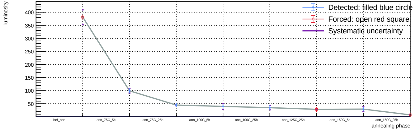
Sensor A1, v = 5 V, T = 23 °C - Spot 65: luminosity vs phase
