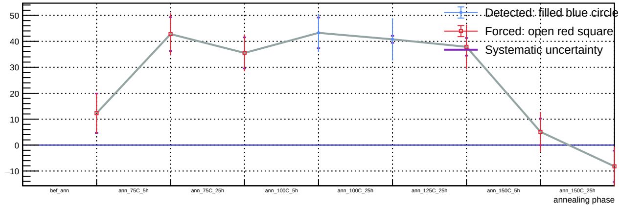
Sensor A1, v = 5 V, T = 23 °C - Spot 66: luminosity vs phase
