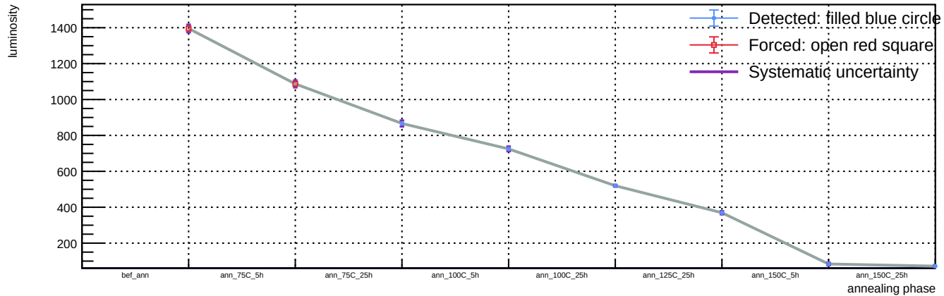
Sensor A1, v = 5 V, T = 23 °C - Spot 67: luminosity vs phase
