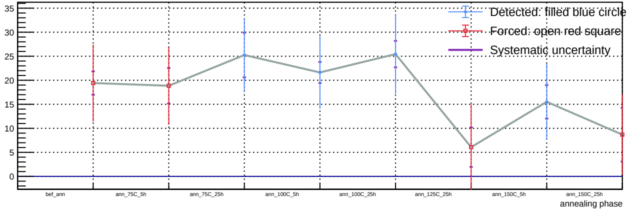
Sensor A1, v = 5 V, T = 23 °C - Spot 68: luminosity vs phase
