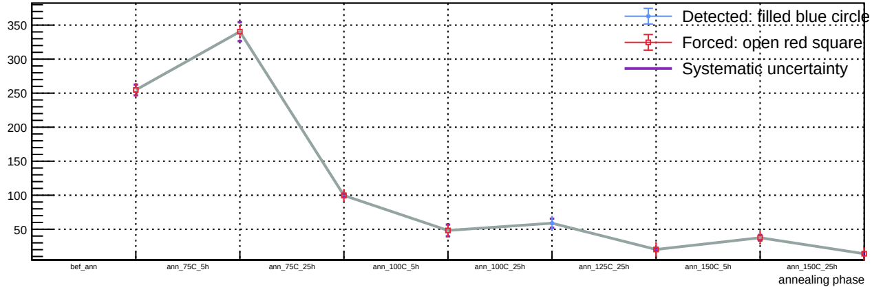
Sensor A1, v = 5 V, T = 23 °C - Spot 69: luminosity vs phase
