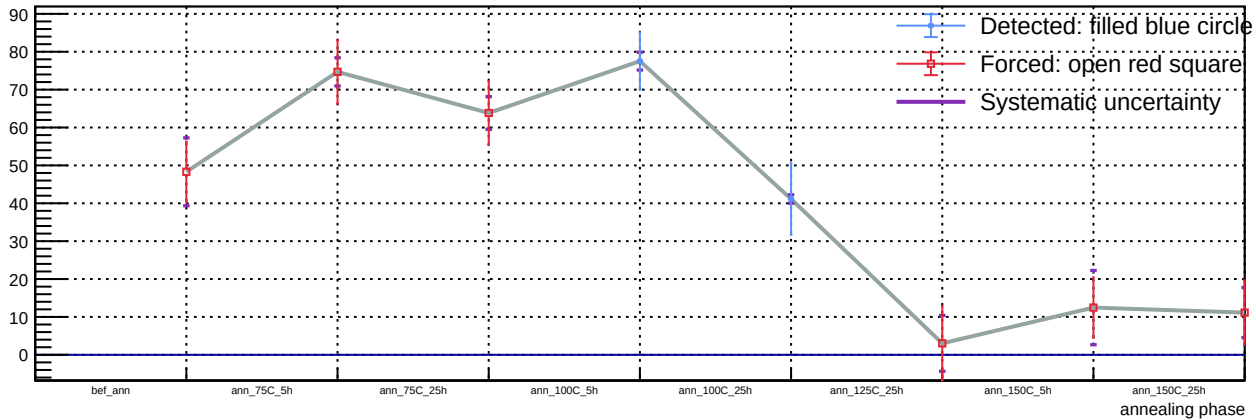
Sensor A1, v = 5 V, T = 23 °C - Spot 71: luminosity vs phase
