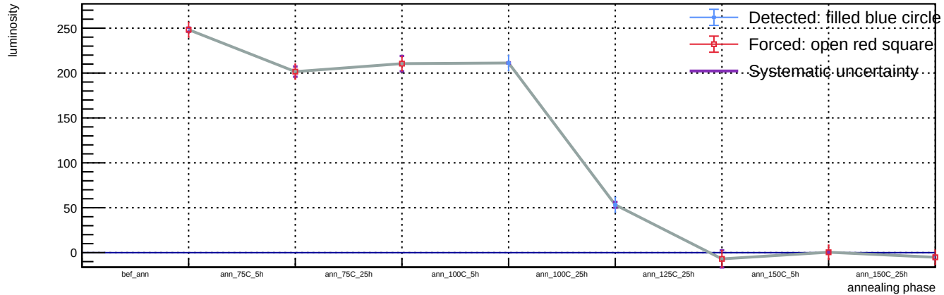
Sensor A1, v = 5 V, T = 23 °C - Spot 72: luminosity vs phase
