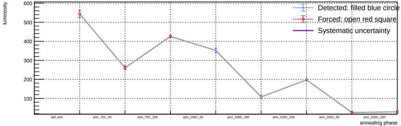
Sensor A1, v = 5 V, T = 23 °C - Spot 73: luminosity vs phase
