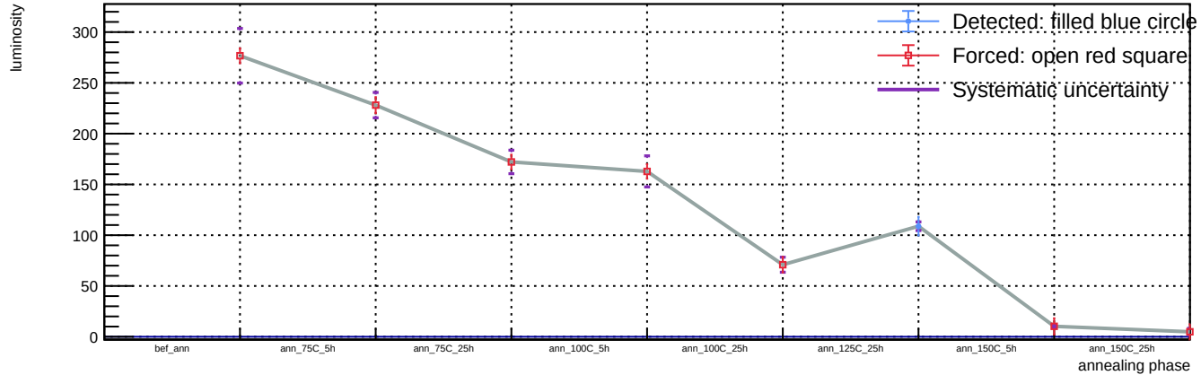
Sensor A1, v = 5 V, T = 23 °C - Spot 75: luminosity vs phase
