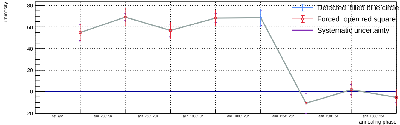
Sensor A1, v = 5 V, T = 23 °C - Spot 79: luminosity vs phase
