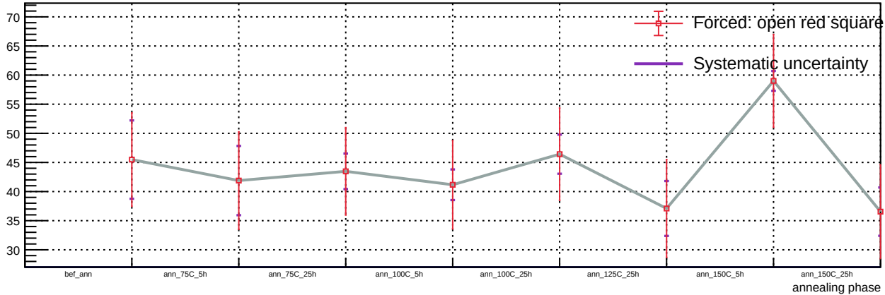
Sensor A1, v = 5 V, T = 23 °C - Spot 80: luminosity vs phase
