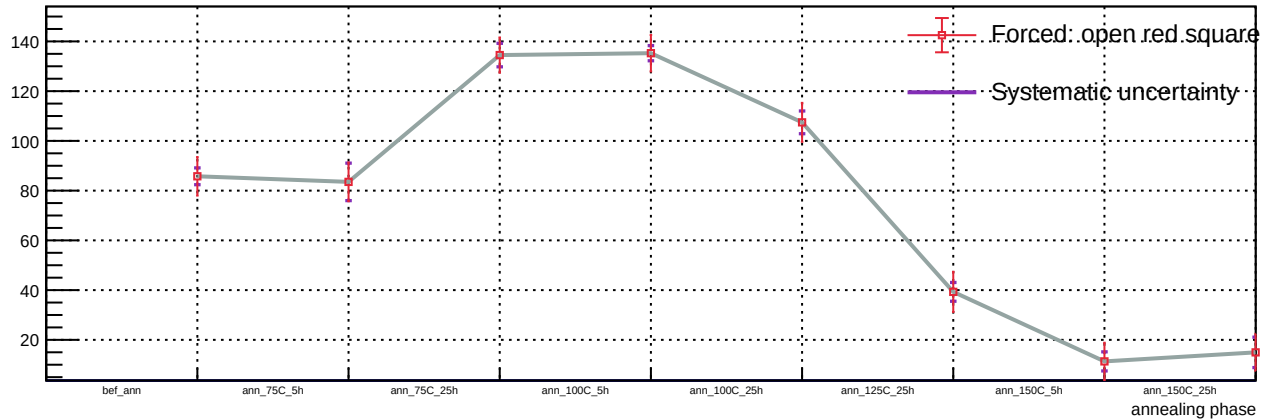
Sensor A1, v = 5 V, T = 23 °C - Spot 82: luminosity vs phase
