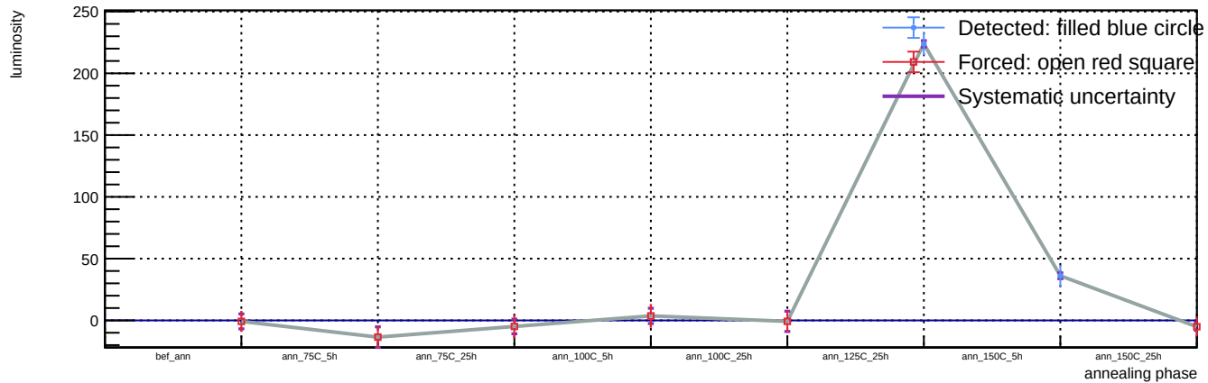
Sensor A1, v = 5 V, T = 23 °C - Spot 83: luminosity vs phase
