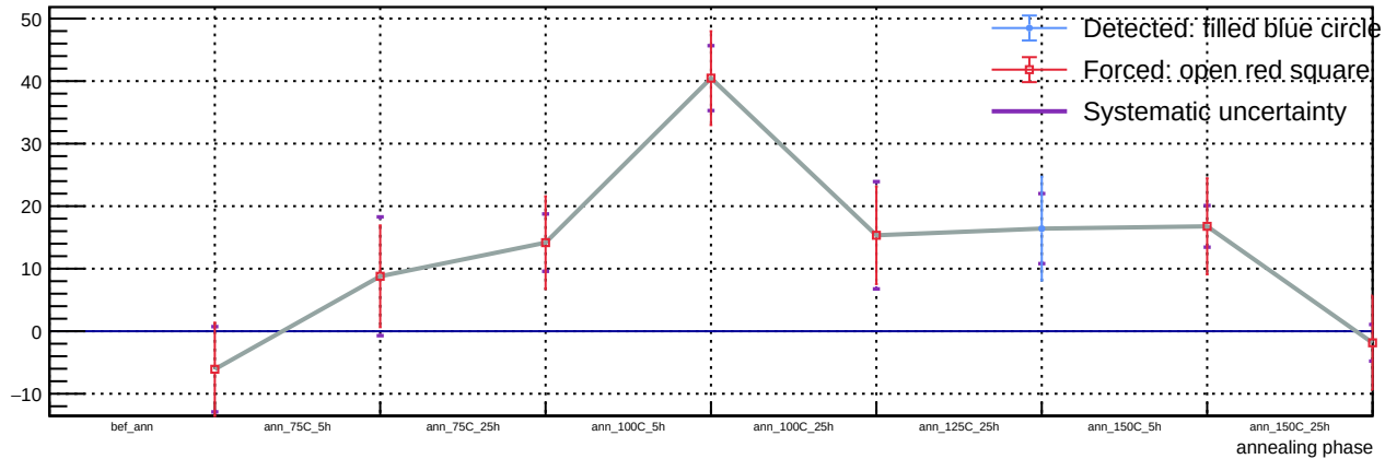
Sensor A1, v = 5 V, T = 23 °C - Spot 84: luminosity vs phase
