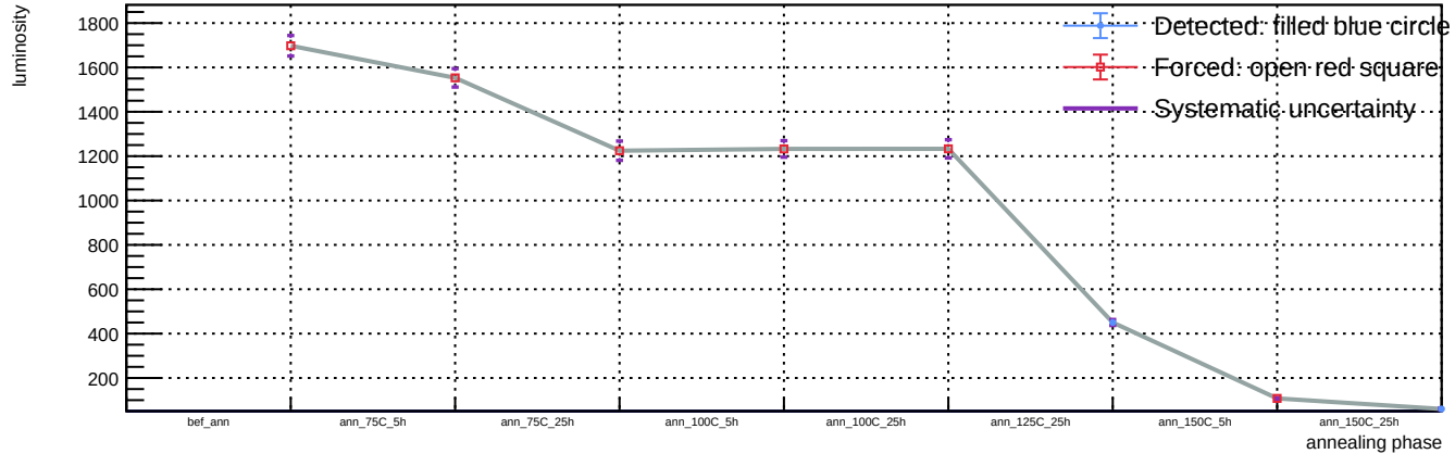
Sensor A1, v = 5 V, T = 23 °C - Spot 85: luminosity vs phase
