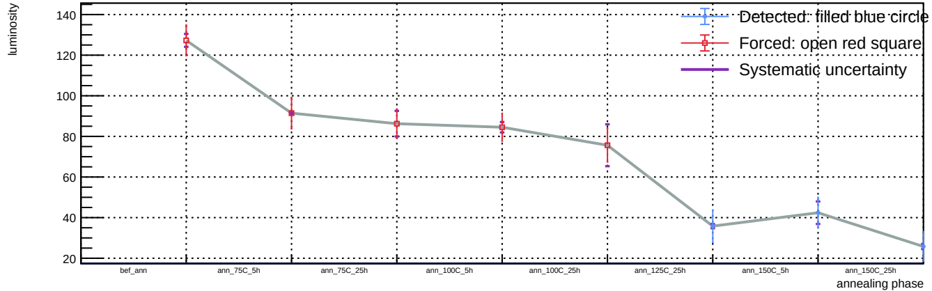
Sensor A1, v = 5 V, T = 23 °C - Spot 86: luminosity vs phase
